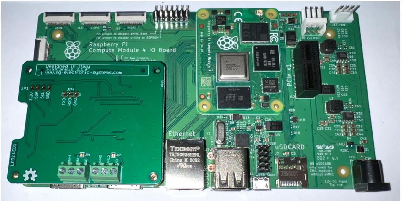
Figure 2-6 Can Bus Dual Base V2.1.4 on CM4
