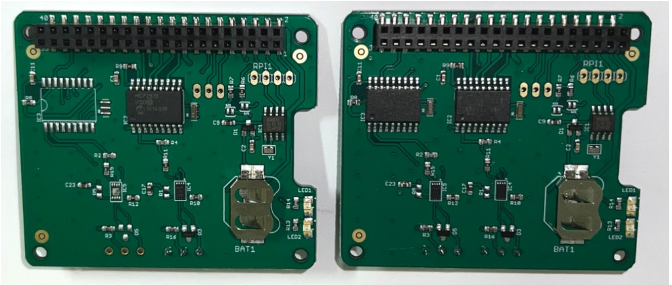
Figure 1-1 Can Bus Dual Base V2.1.4 One Channel (Left) Two Channels (Right)
