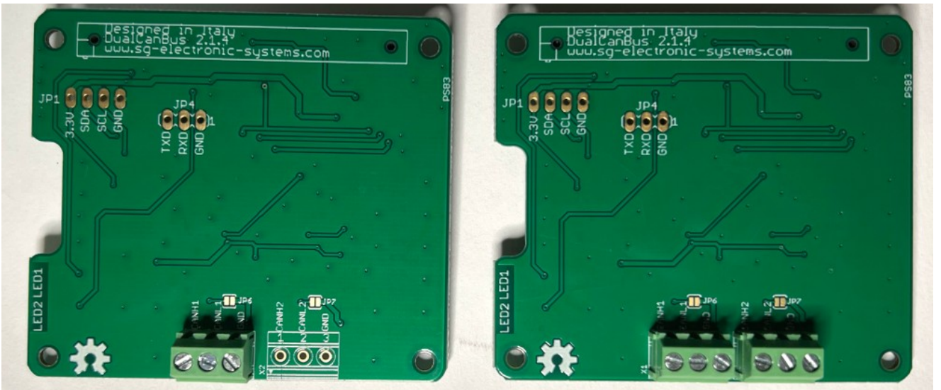
Figure 1-2 Top side Can Bus Dual Base V2.1.4 One Channel (Left) Two Channels (Right)
